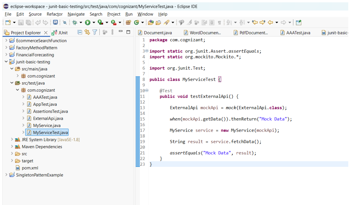
Figure 8: MyServiceTest Implementation
